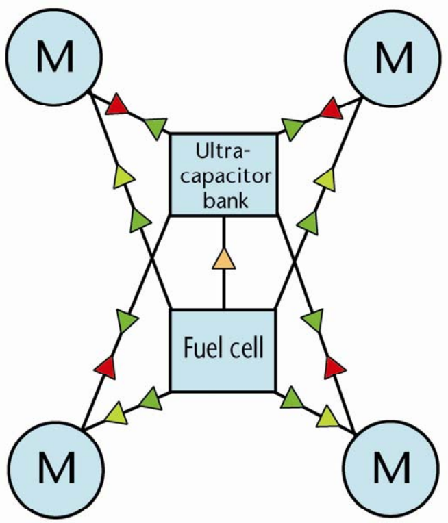
The network electric powertrain
